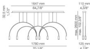
VP43114C Metal+Aluminum L1780*W125*H2600mm LED
