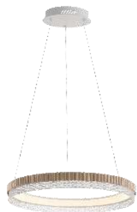
3275-P40/50/60 Color: Black/White/Gold Iron+PS D400/500/600*H1500MM LED 40/50/60W
