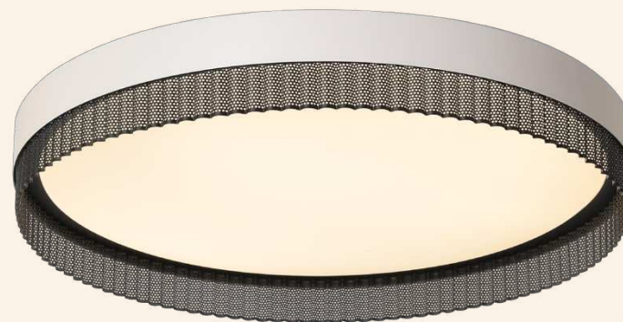
DH-8239WB-CS/M/L/XL ø323*95 ø427*95 ø515*95 ø625*95 LED IP20
